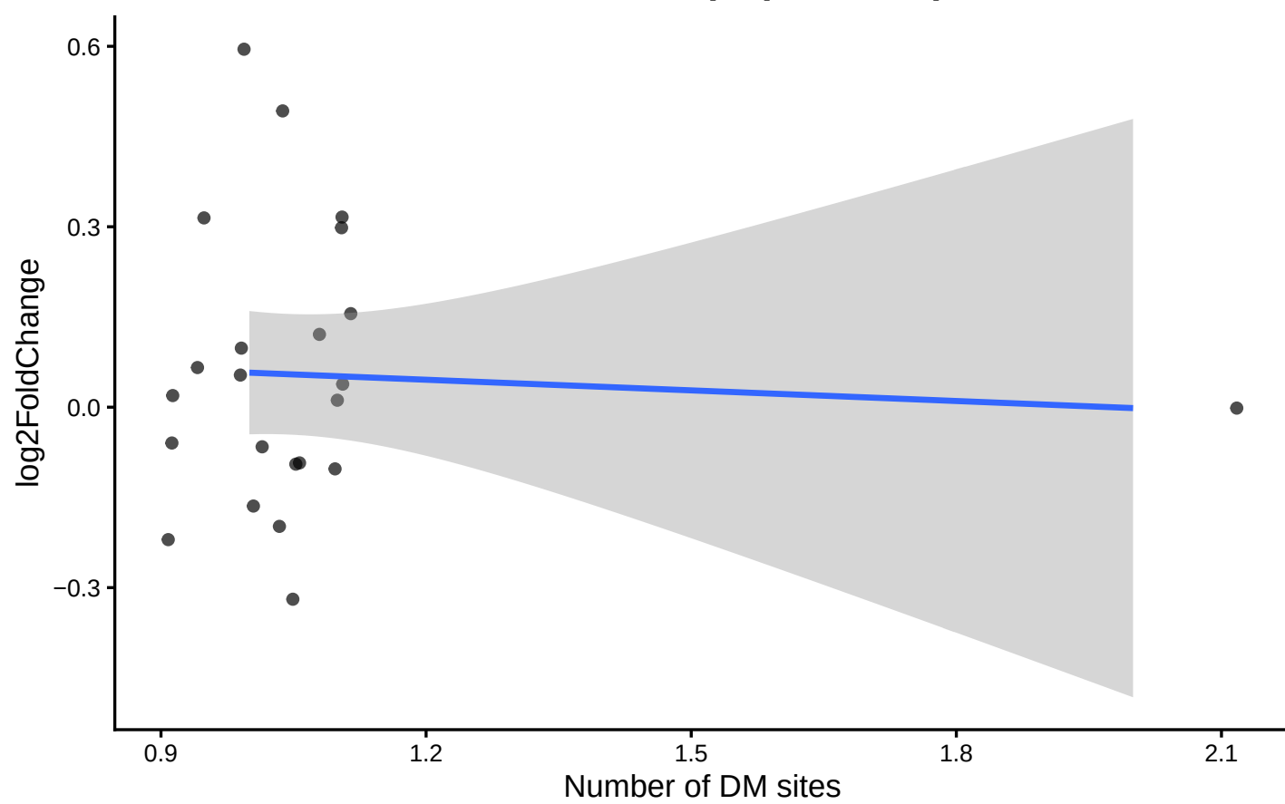
M3: Correlation # DM sites vs expr (direction)
