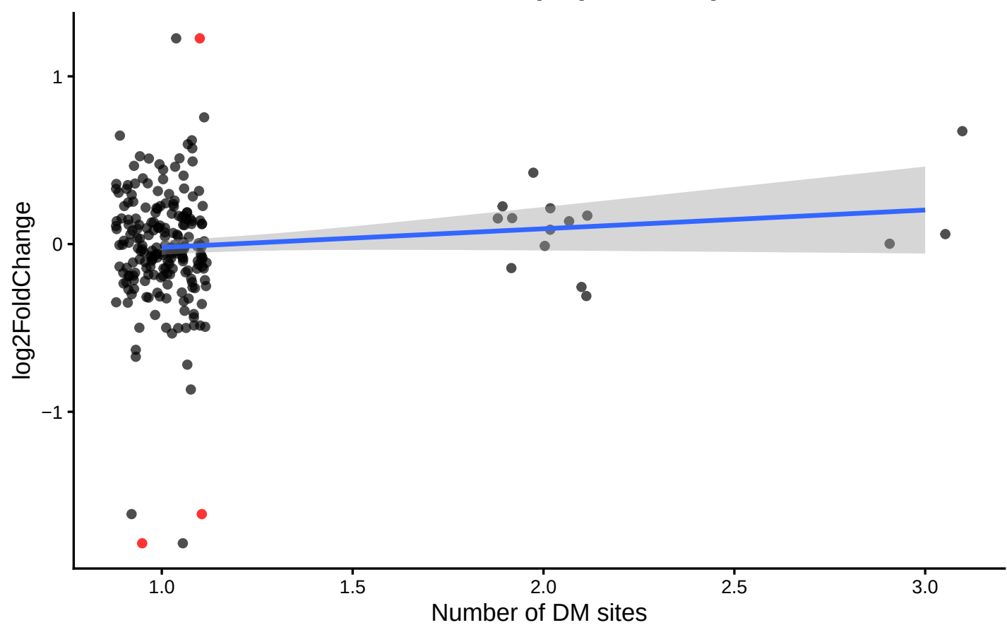
M5: Correlation # DM sites vs expr (direction)
