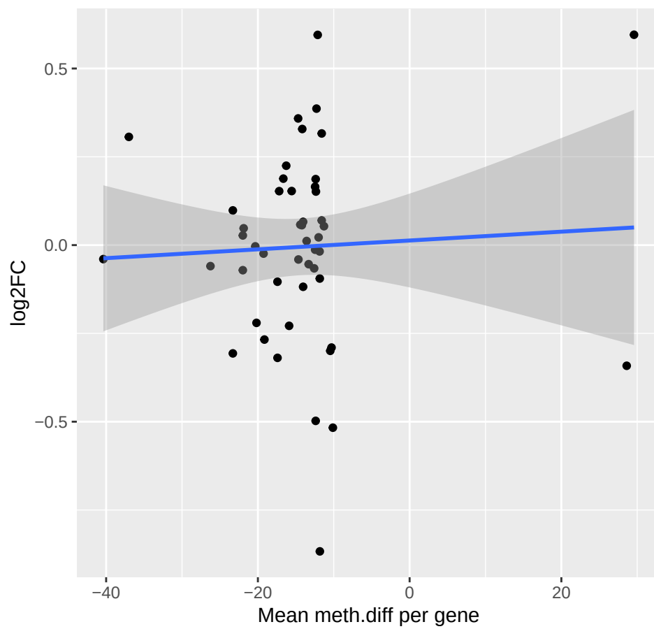
M4: Body methylation vs Expression
