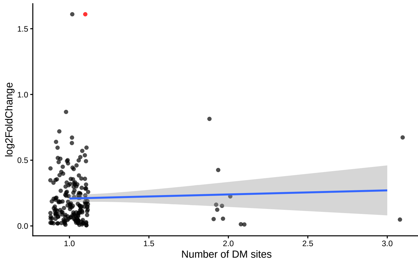
M1: Correlation # DM sites vs expr (direction)
