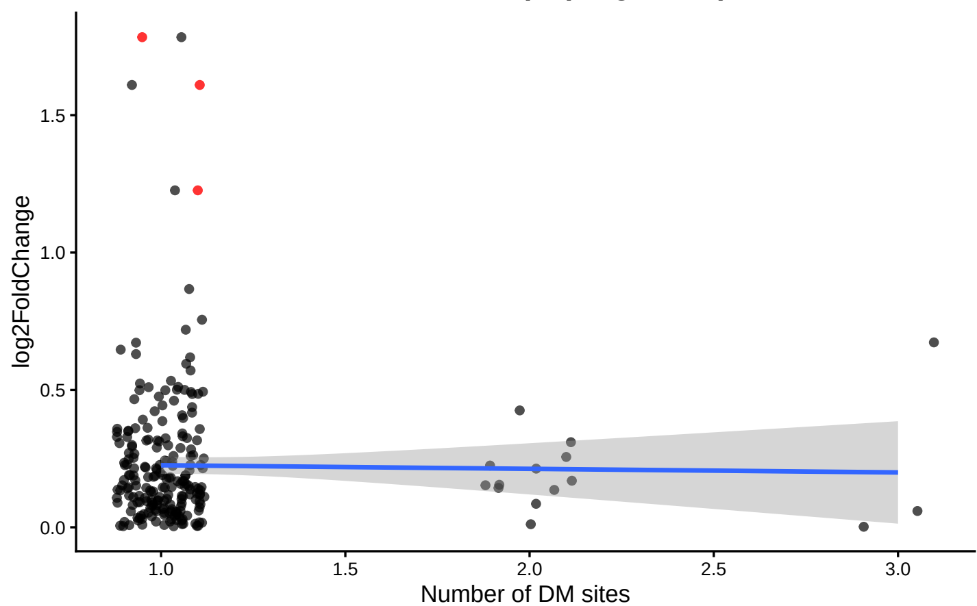
M5: Correlation # DM sites vs expr (magnitude)
