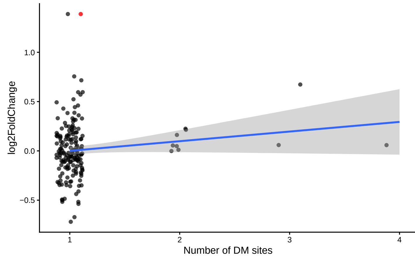
M2: Correlation # DM sites vs expr (direction)
