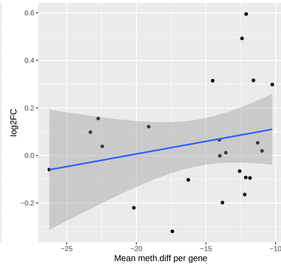
M3: Body methylation vs Expression
