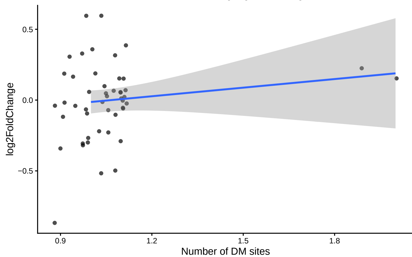
M4: Correlation # DM sites vs expr (direction)
