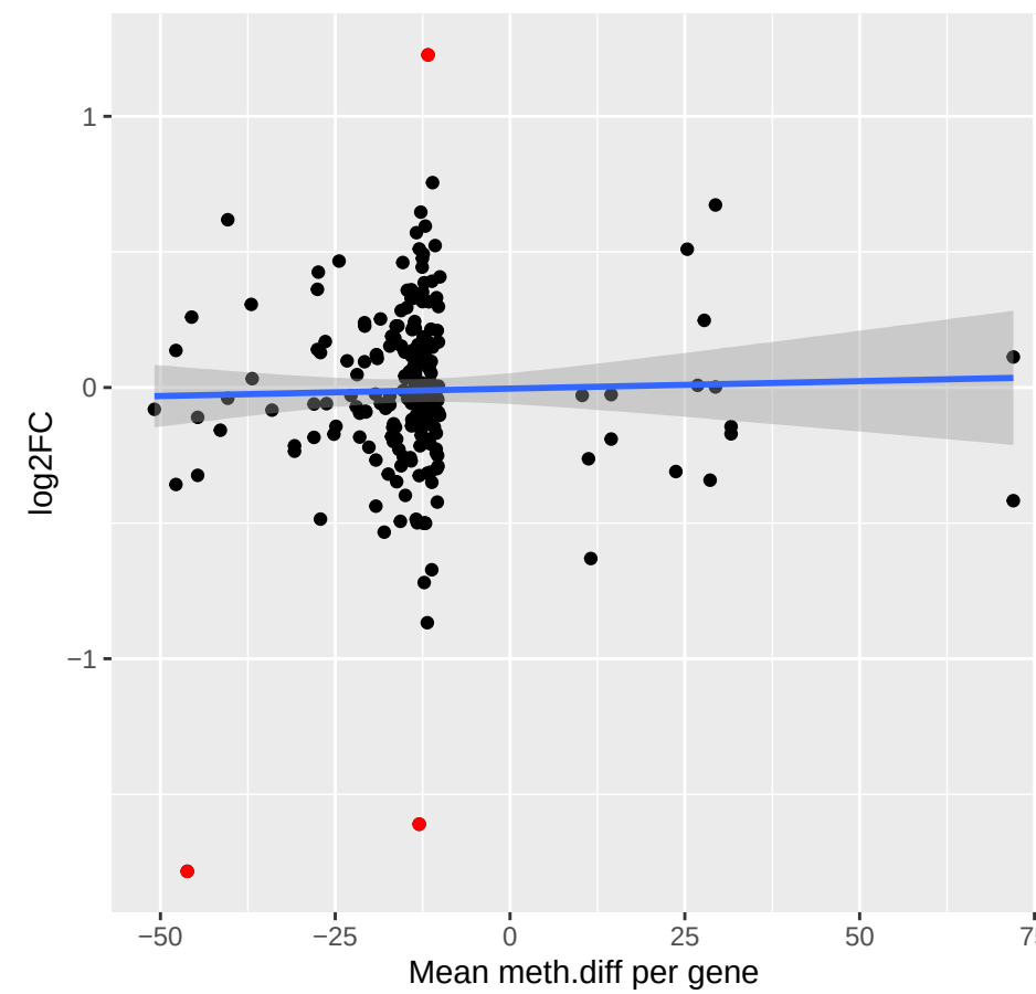
M5: Body methylation vs Expression
